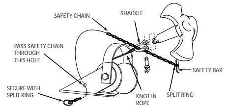
Figure 4. Anchor Attachment
