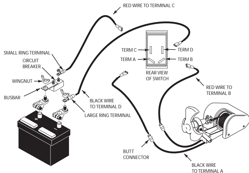
Figure 2. Pan Fisherman Wiring
